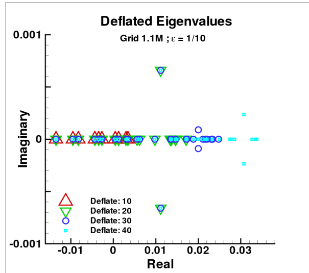
Figure 3. Comparison of eigenvalues obtained using 10, 20, 30, and 40 enrichment vectors. The Krylov dimension is 60 in all cases. Preconditioner is ILU(1) .
