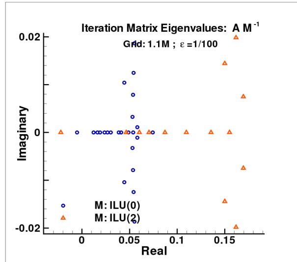
Figure 5. Advection-diffusion eigenvalues located near the origin for the parameter \epsilon = \frac{1}{100} with two preconditioners ILU(0) and ILU(2) .
