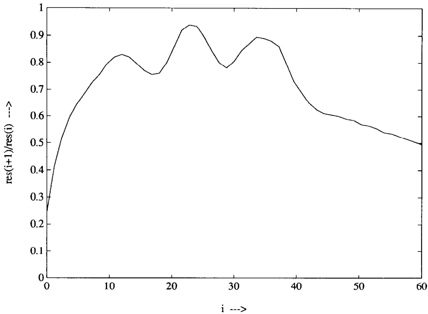
Fig. 4. GMRES for a spectrum with a Jordan block of size 3.
