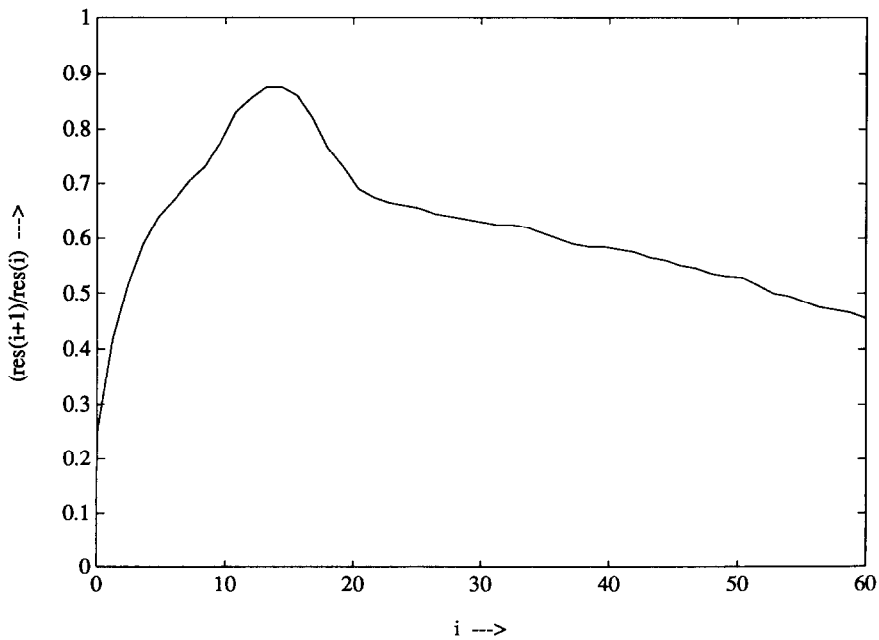
Fig. 3. GMRES for a spectrum with multiple eigenvalues.
