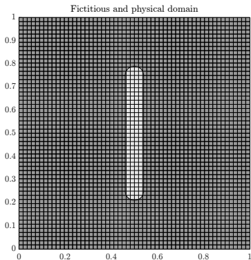
(a) Fictitious domain \hat{\Omega} (light gray) and physical domain \Omega (dark gray)
