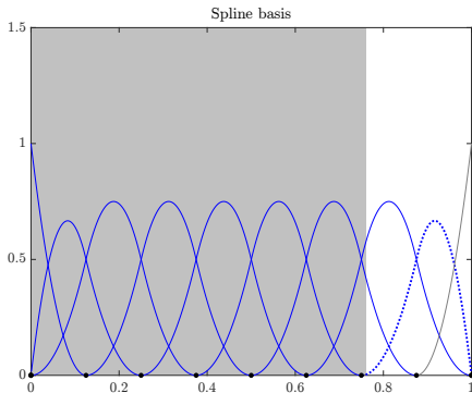
(a) C^1 smoothness
