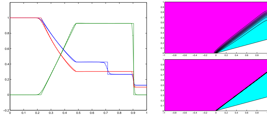
Figure 2. Shock tube problem (left) and compression corner (right)
