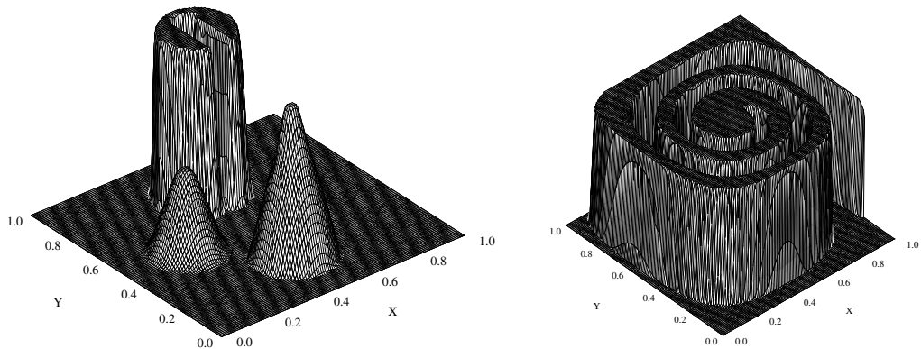
Figure 1. Solid body rotation (left) and swirling flow (right).
