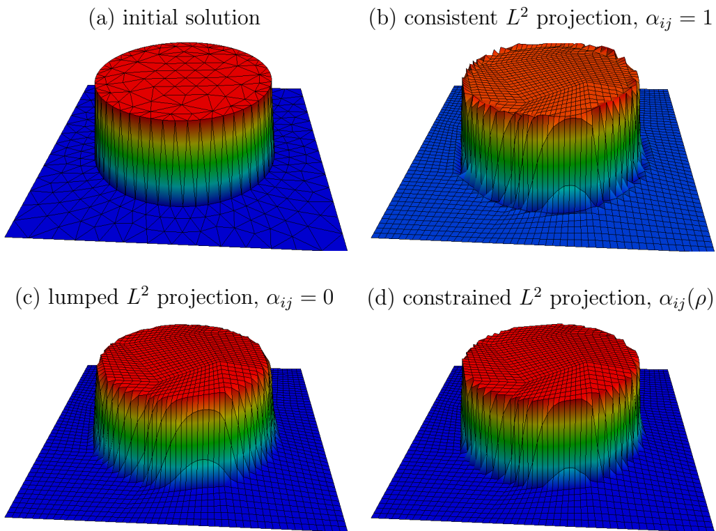
Fig. 10. Constrained interpolation: initial and interpolated solutions.
