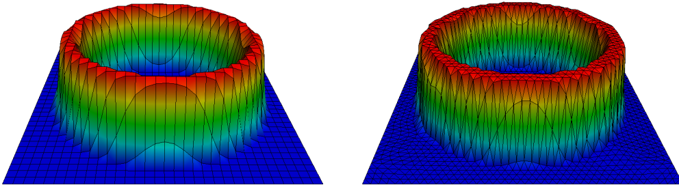
(c) constrained L^2 projection, \alpha_{ij}(\rho)
